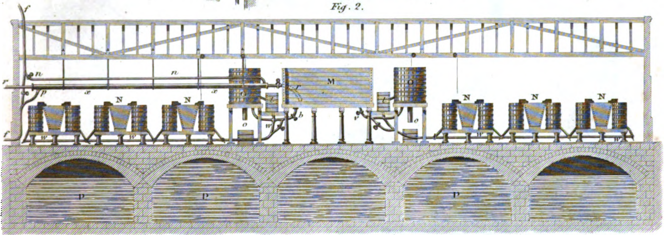
Malt rollers
