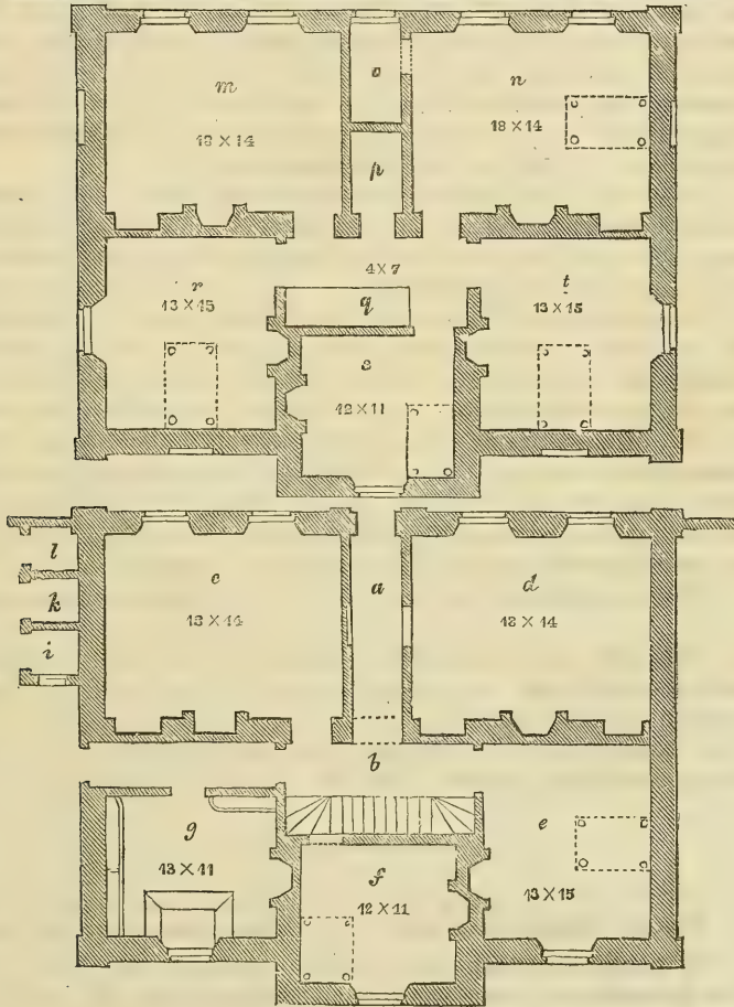
The Ground Floor contains: a , entrance lobby; b , passage and staircase; c , kitchen; d , parlour; e , apprentice's bed-room; f , servant's bed-room; g , office and library; i , l , water-closets; k , fuel; l , ashes. The Chamber Floor contains: m , seed room over the kitchen; n , best bed-room; o , closet to best bed-room; p , lumber closet; q , press for linen; r , s , t , bed-rooms.
