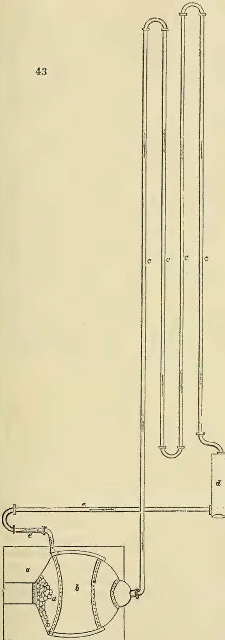
a, Furnace, section. b, Boiler. c c c c, Hot-water tubes. d, Expansion tube. e e, Return- ing tube.
