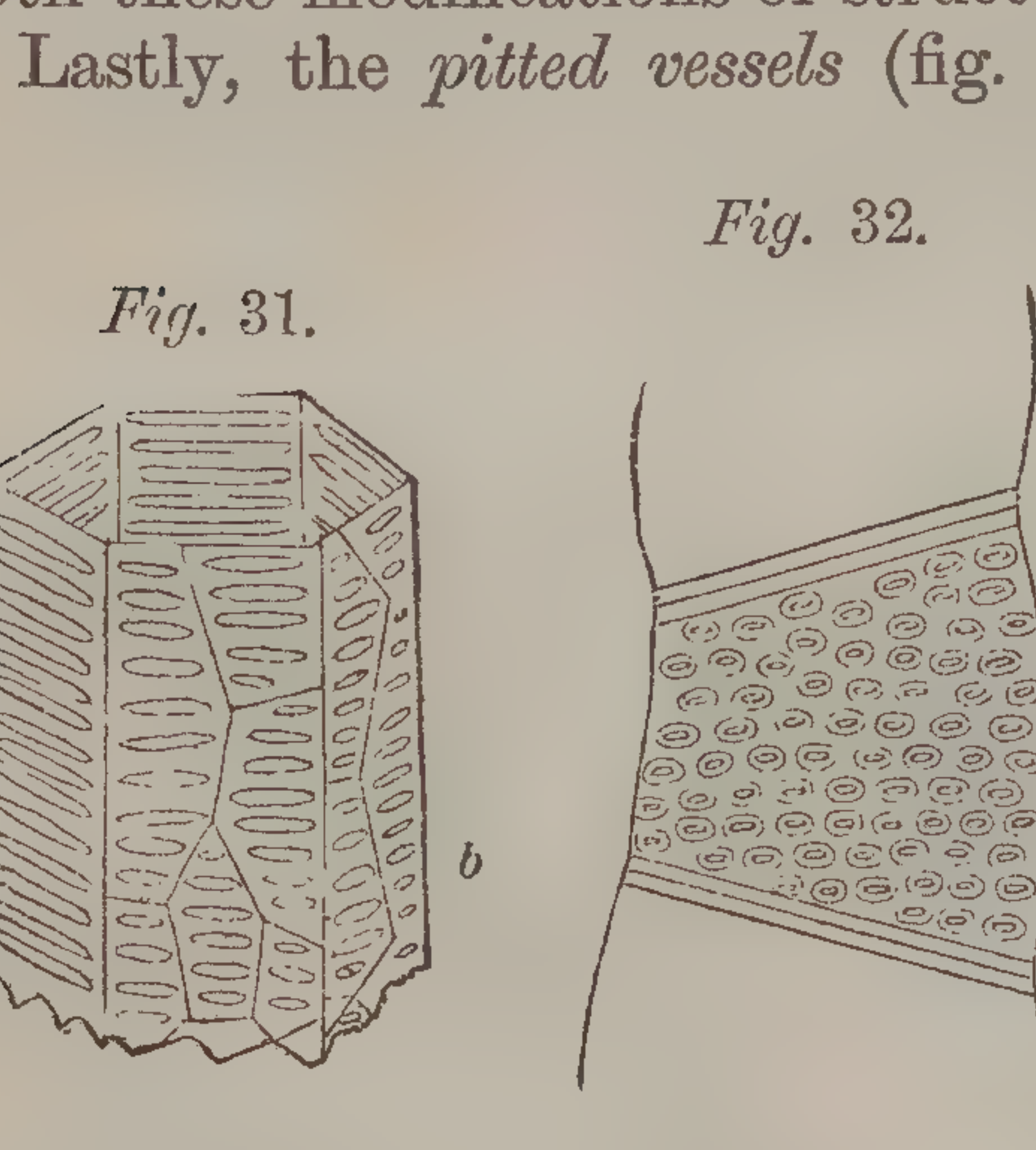
Reticulated vessel from a tree Fern.
