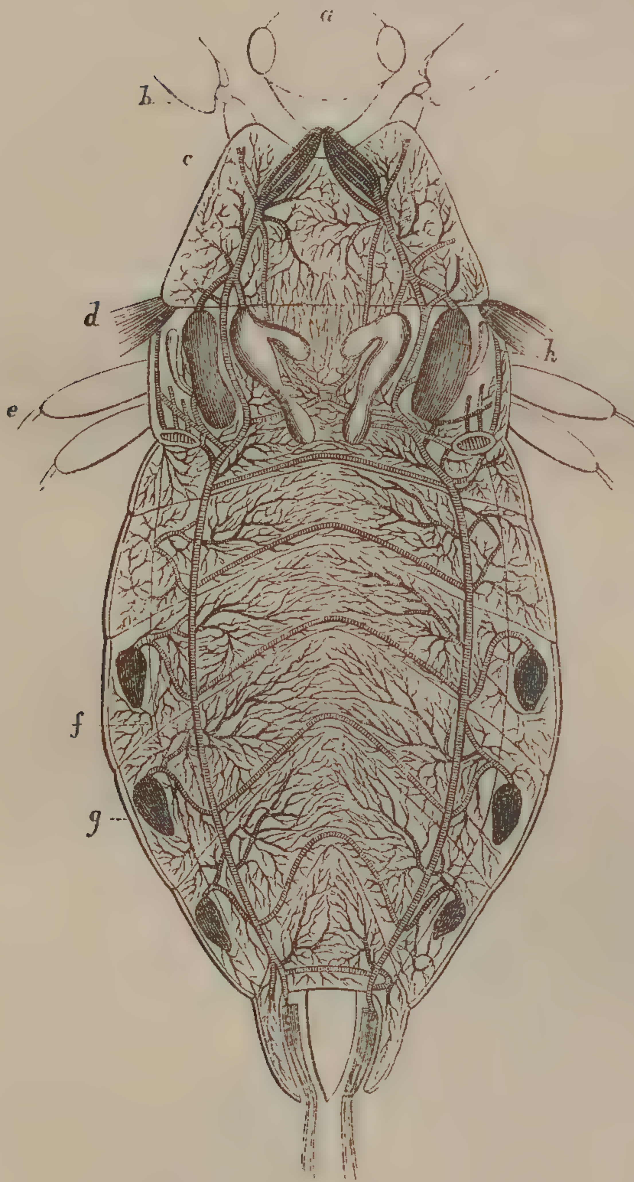
Tracheal system of Nepa (Water-Scorpion):— a , head; b , first pair of legs; c , first segment of the thorax; d , second pair of wings; e , second pair of legs; f , tracheal trunk; g , one of the stigmata; h , air-sac.
