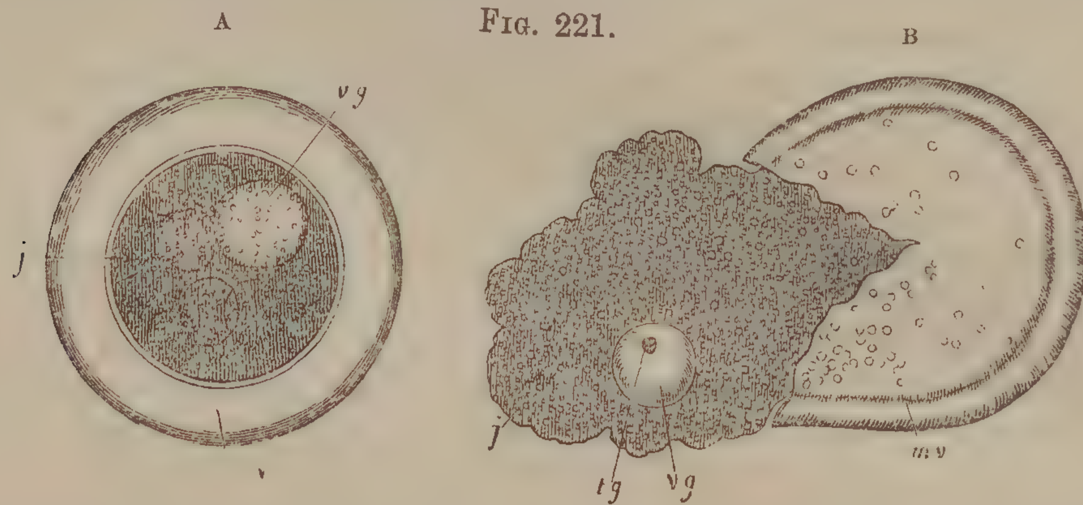
Constituent parts of Mammalian Ovum :—A, entire; B, ruptured, with the contents escaping; — mv , vitelline membrane; f , yolk; vg , germinal vesicle; tg , germinal spot.
