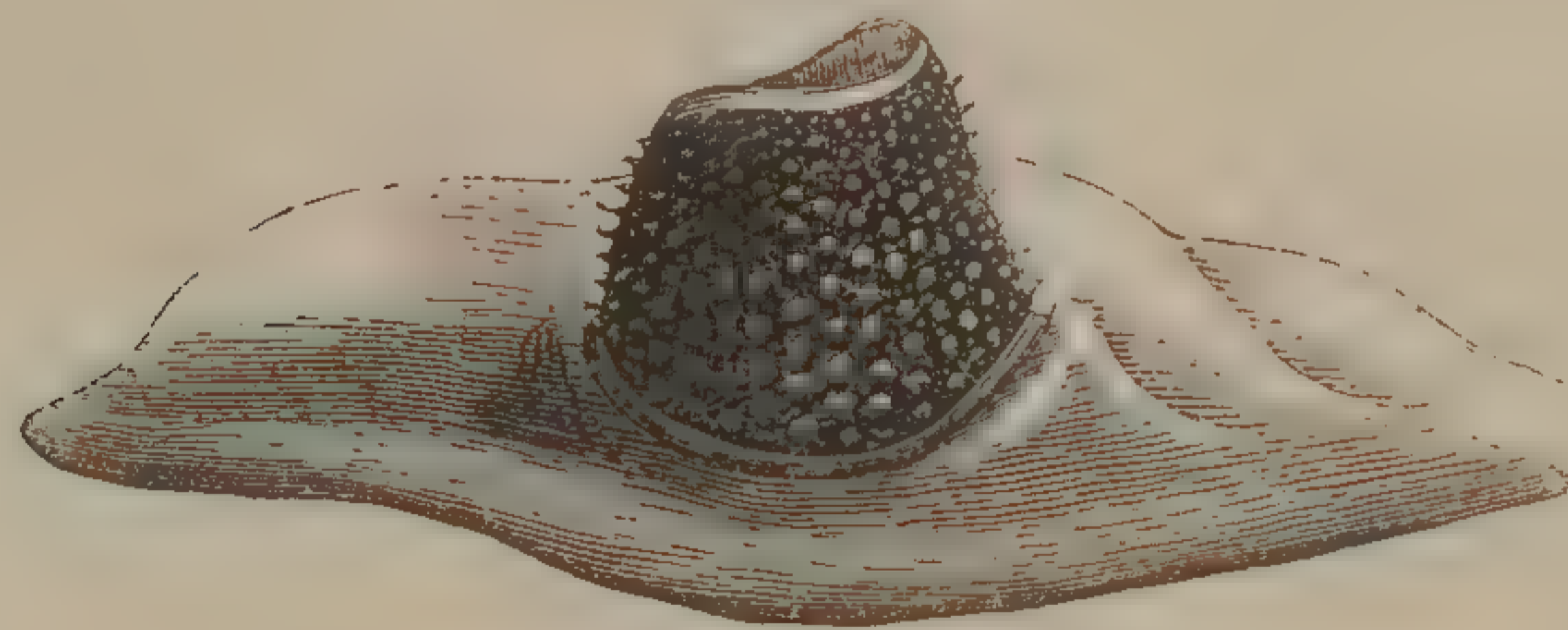
Faceted eye of Asaphus caudatus .
