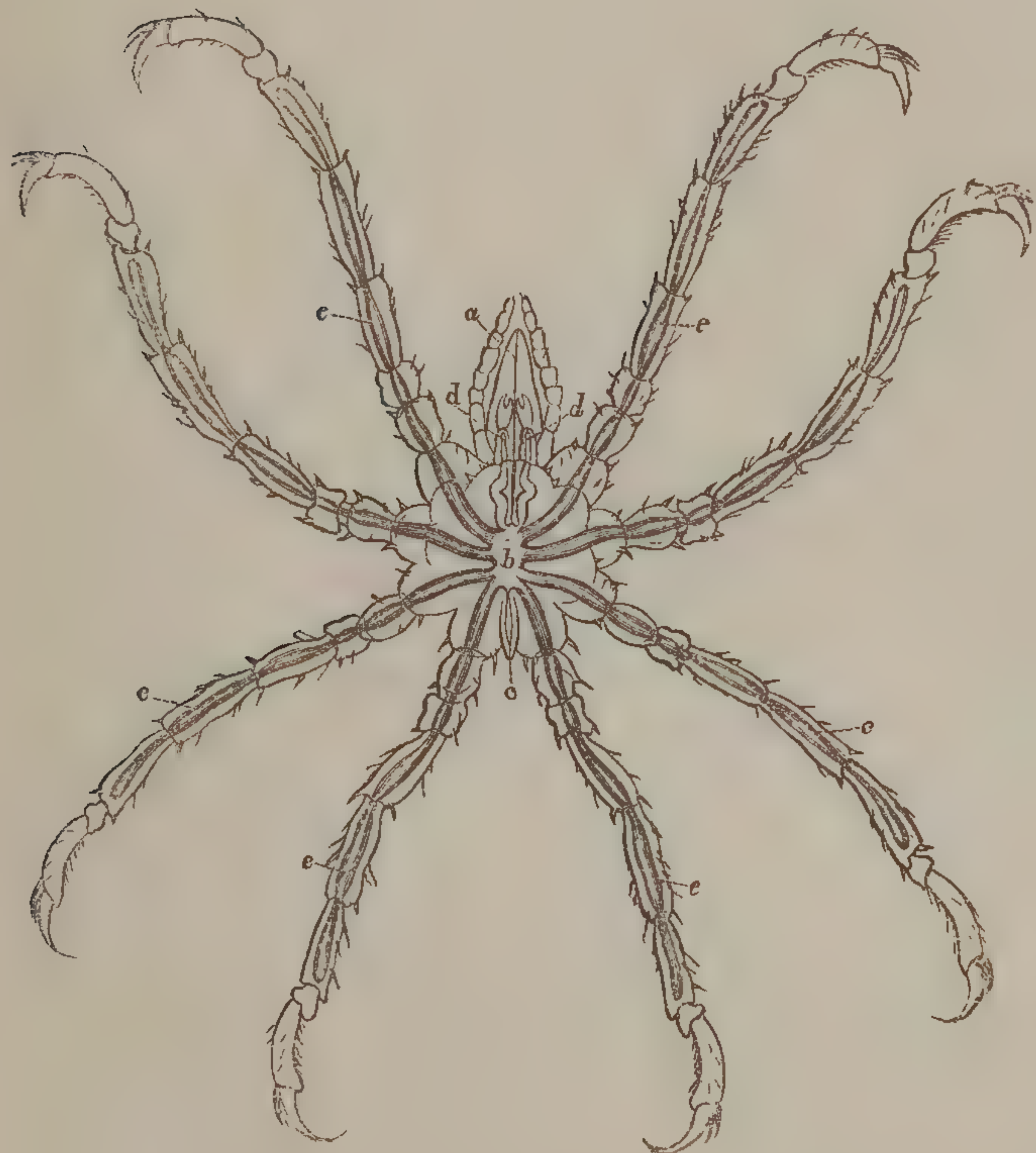
Ammothea pycnogonoides ;— a , narrow oesophagus; b , stomach; c , intestine; d , digestive cæca of the feet-jaws; e e , digestive cæca of the legs.
