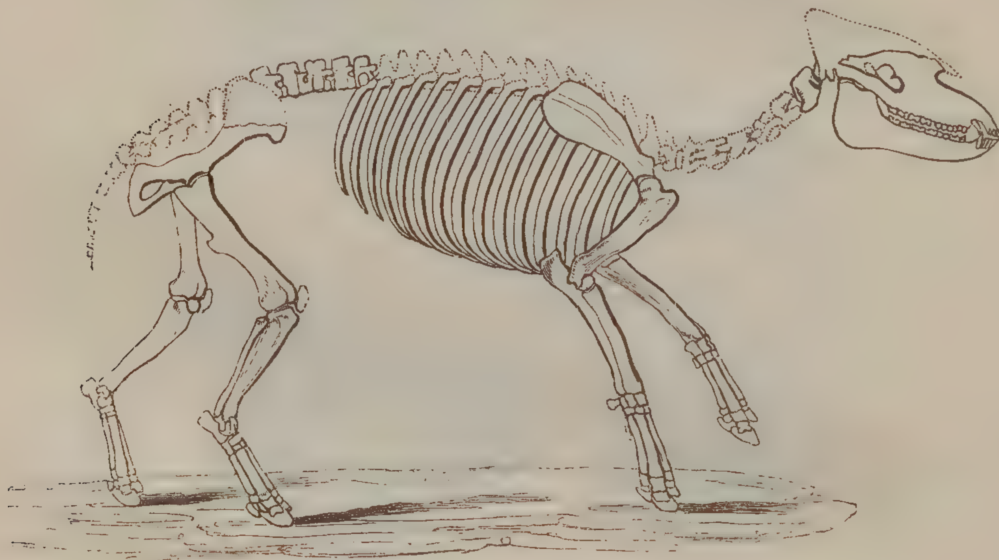
Skeleton of Palæotherium magnum .
