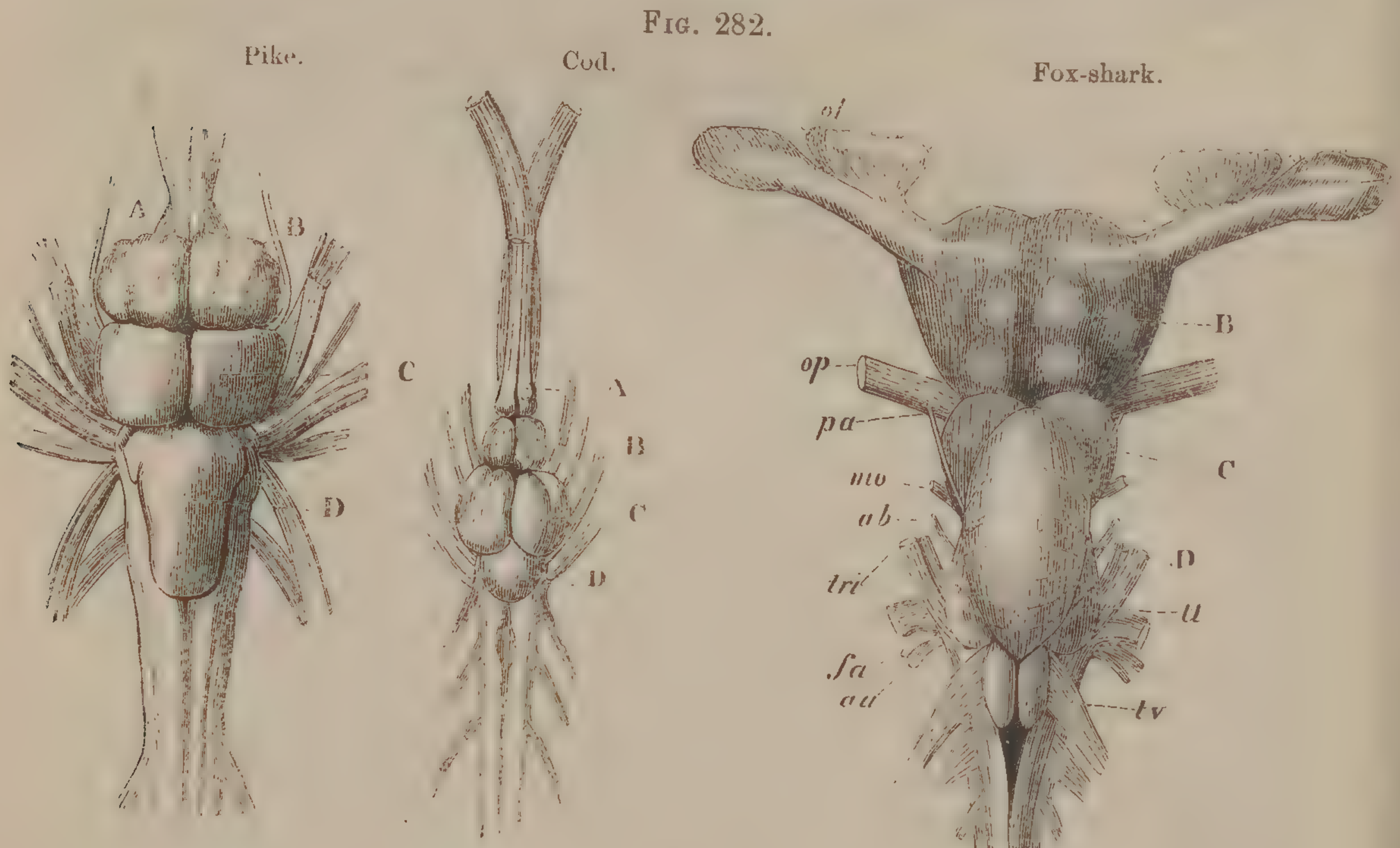
Brains of Fishes :—A, olfactory lobes or ganglia; B, cerebral hemispheres; C, optic lobes; D, cerebellum;— ol , olfactory nerve; op , optic nerve; pa , patheticus; mo , motor oculi; ab , abducens; tri , trifacial; fa , facial; au , auditory; vag , vagus; tt , tubercles or ganglia of the trifacial; tv , tubercles of the vagus.
