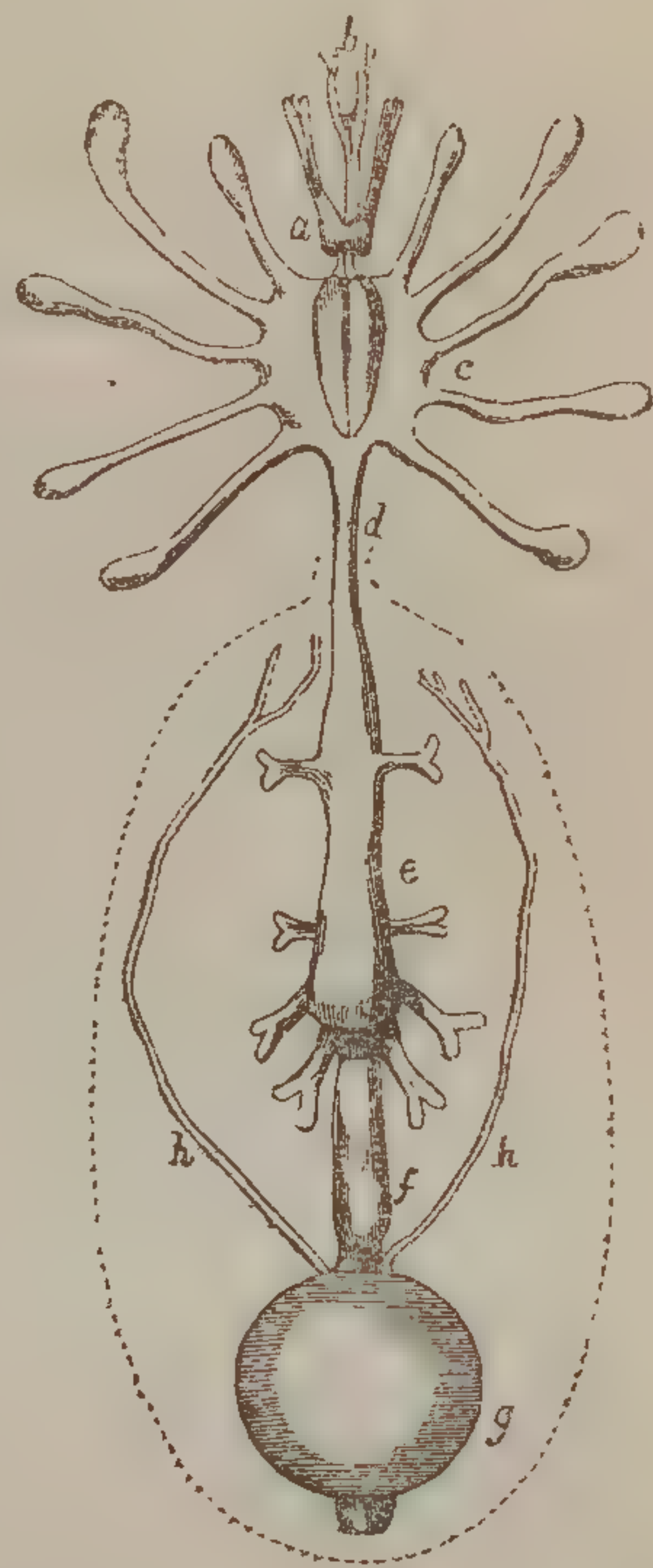
Digestive apparatus of Mygale :— a , cephalic ganglion; b , bifurcated origin of oesophagus; c , stomach with lateral cæca passing into the limbs and palpi; d , portion which traverses the abdominal peduncle; e , dilated intestine, receiving biliary vessels; f , small intestine; g , caecal enlargement, receiving the urinary vessels h, h .
