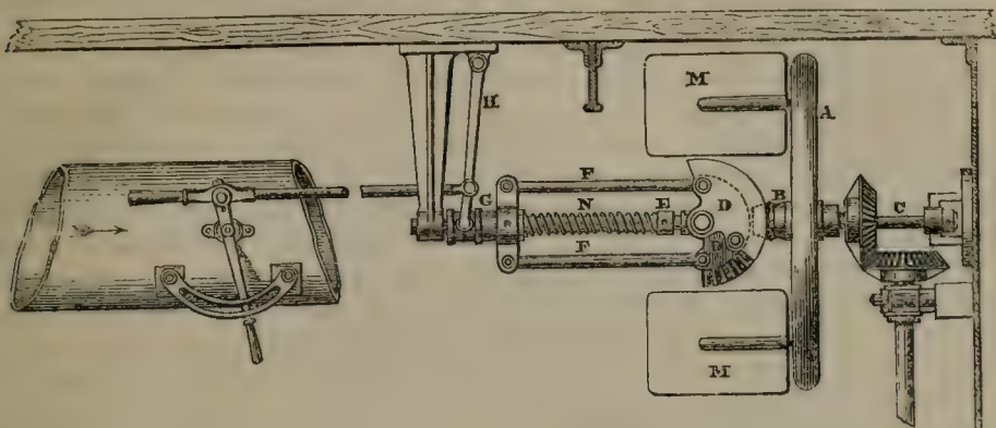
Silver's Patent Marine and Stationary Engine Governors. Constructed by John Hamilton, Engineer, Glasgow.
