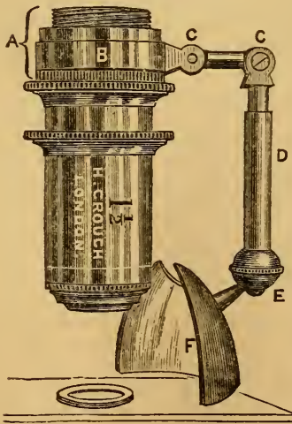
Crouch's Adapter for Parabolic Speculum.
