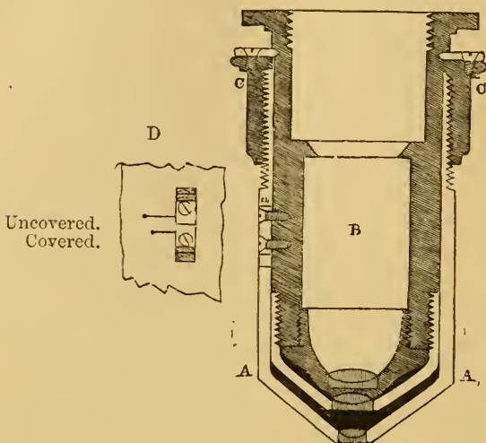
Section of an Adjusting Object-Glass.
