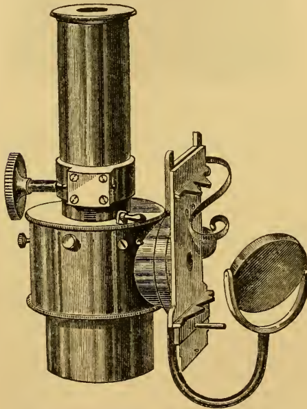
Sorby-Browning Spectroscope Eye-piece.
