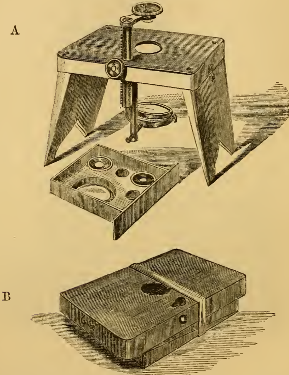
Quekett's Dissecting Microscope, set up for use at A, and packed together at B.
