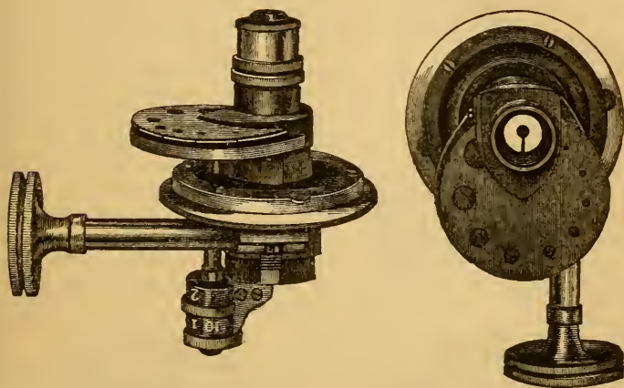
Powell and Lealand's Achromatic Condenser.
