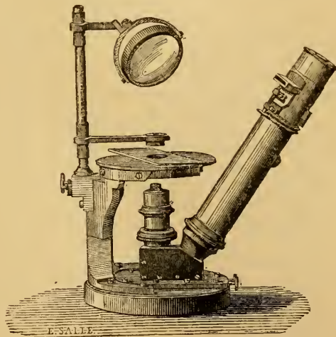
Dr. Lawrence Smith's Inverted Microscope.
