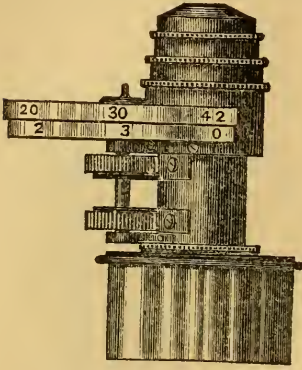
Ross's Achromatic Condenser.
