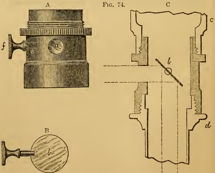
Beck's Vertical Illuminator.
