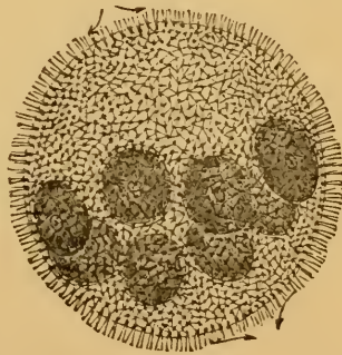
Volvox Globator.
