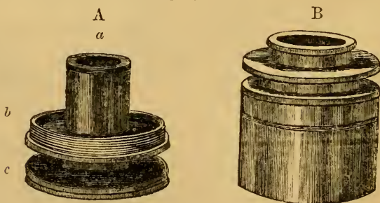
Fitting of Polarizing Prism in Smith and Beck's Microscope.
