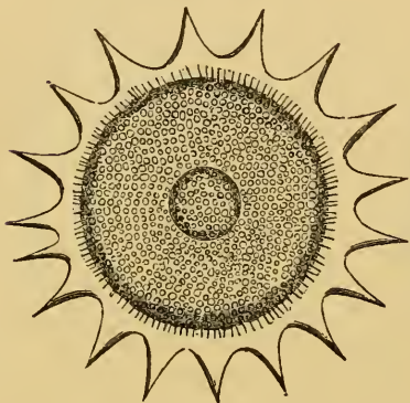
Haliomma Humboldtii.
