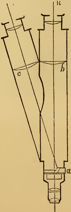
Wenham's Stereoscopic Binocular Microscope.
