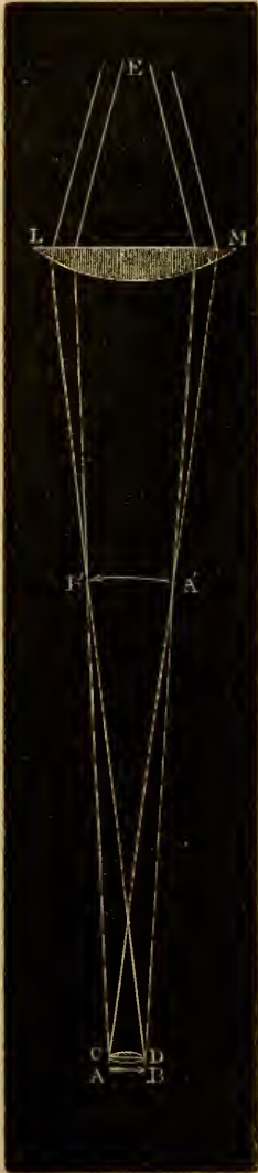
Diagram of simplest form of Compound Microscope.
