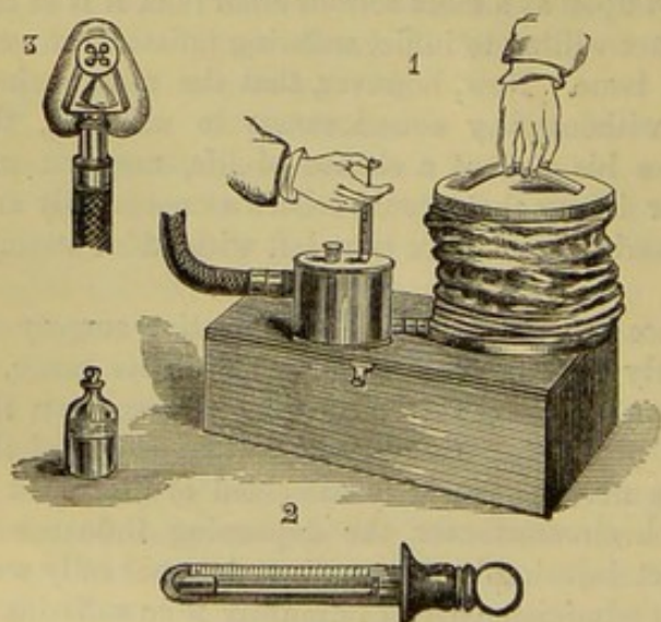
Fig. 1.—Clover's Chloroform Apparatus.
