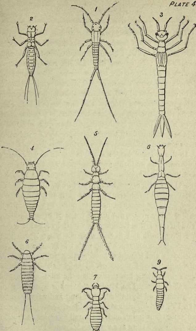
PLATE IV. YOUNG FORMS OF THE INSECTS REPRESENTED ON PLATE III.—Fig. 1, Larva of Chloëon ; 2, Larva of Meloe (after Chapuis and Candère) ; 3, Larva of Calepteryx (after Léon Dufour) ; 4, Larva of Sitaris ; 5, Larva of Campodea ; 6, Larva of Acilius ; 7, Larva of Termes (after Blanchard) ; 8, Larva of Stylops ; 9, Larva of Thrips.
