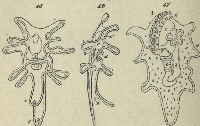
FIG. 45, Larva of Starfish ( Bipinnaria ), \times 100 (after Müller). 46, Larva of Starfish ( Bipinnaria ), \times 100 , seen from the side— a , mouth; b , œsophagus; c , stomach; c' , intestine. 47, Larva of another Bipinnaria , showing the commencement of the Starfish— g , canal of the ciliated sac; i , rudiments of tentacles; k , ciliated band.
