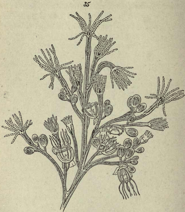
FIG. 35.—Portion of colony of Bougainvillea fruticosa , more magnified.
