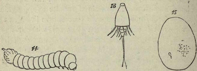
FIG. 14. Larva of Sirex (Westwood, loc. cit.) 15, Egg of Rhynchites , showing the parasitic Larva in the interior. 16, the parasitic Larva more magnified.
