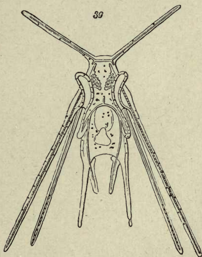
FIG. 39.—Larva of Echino-cidaris, seen from above \times \frac{6}{13} (after Müller).
