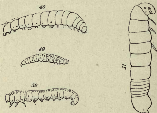
FIG. 48, Larva of Moth ( Agrotis suffusa ), after Packard. 49, Larva of Beetle ( Haltica ), after Westwood. 50, Larva of Sawfly ( Cimbex ), Brischke and Zaddach Beob ub d arren. der Blatt und Holzwespen, Fig. 8. 51, Larva of Julus . Newport, Phils. Transactions, 1841.
