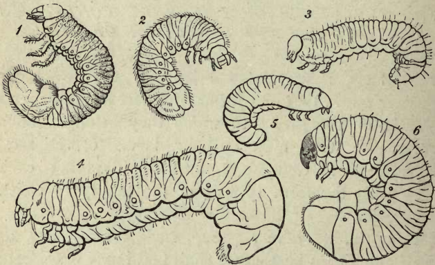
FIG. 1, Larva of the Cockchafer ( Melolontha ). (Westwood, Int. to the Modern Classification of Insec s vol. i. p. 194.) 2, Larva of Ceton a . 3, Larva of Trux . 4, Larva of Oryctes . 5, Larva of Aphodius (Chapuis and Candèz, Mém. Soc. Roy. Liège, 1853). 6, Larva of Lucanus (Packard, Guide to the Study of Insects, Fig. 403).
