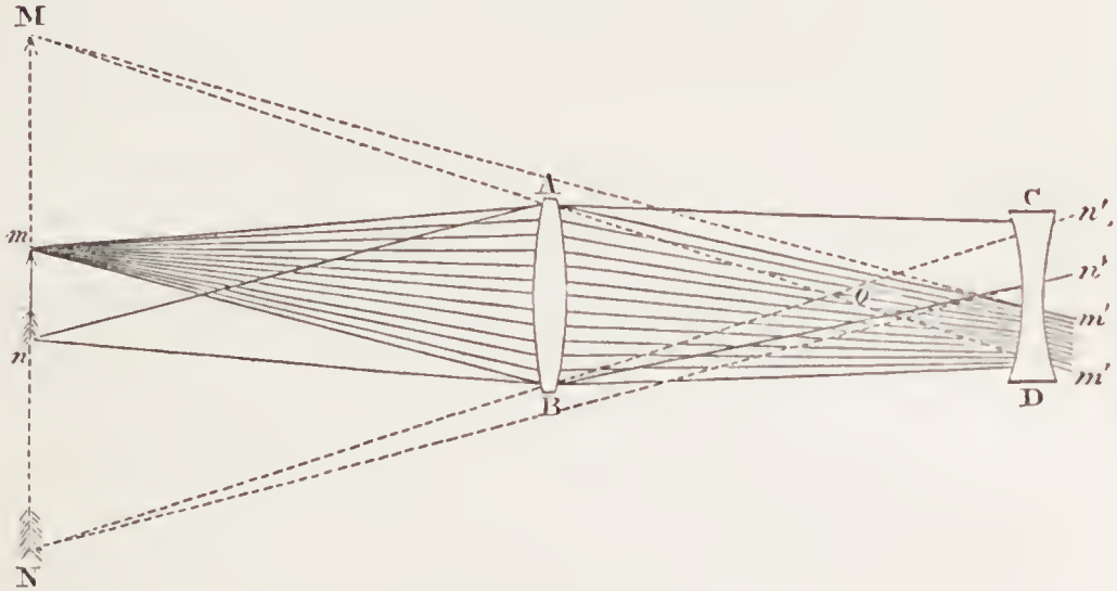
Galileo's Telescope.
