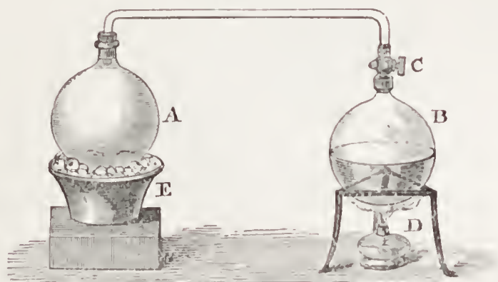
Steam condensed in a separate Vessel.
