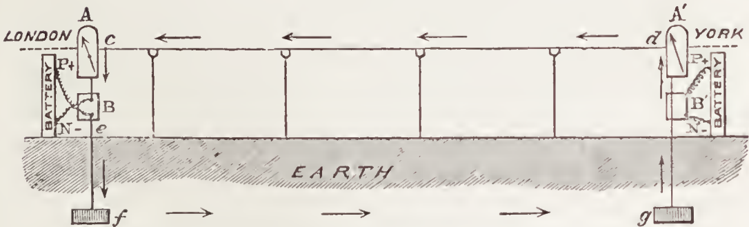
Diagrams showing the general principle of the Electric Telegraph.
