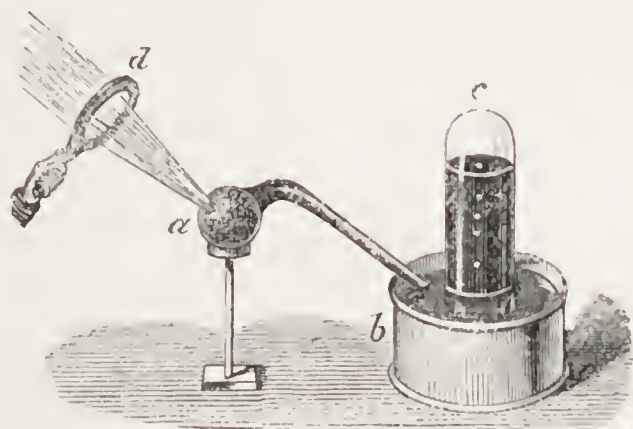
Priestley's Apparatus for procuring Oxygen.
