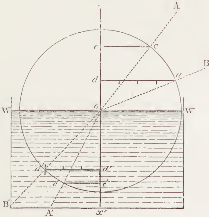
Measurement of Refraction in Water.
