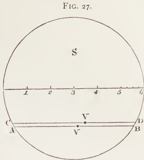
Transit of Venus.
