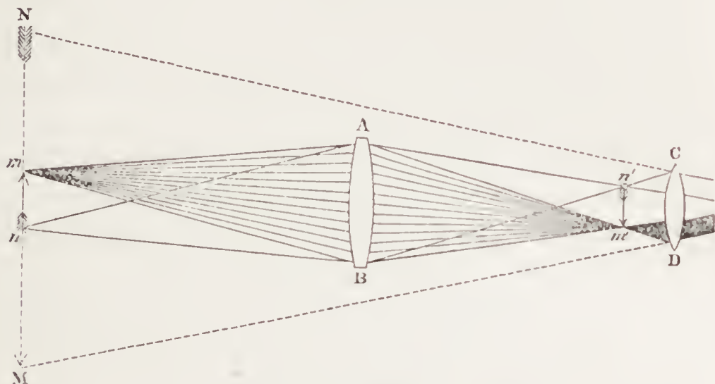
Kepler's Telescope. 1
