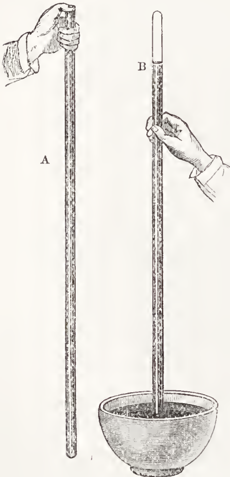
Torricelli's Experiment (Ganot).
