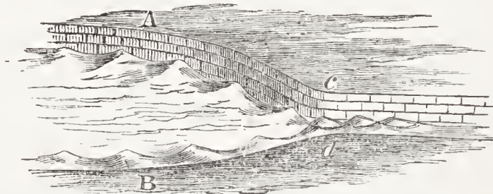
Diagrams illustrating the Interference of Waves.
