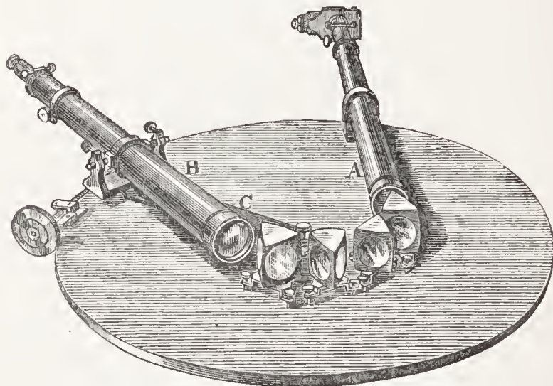
Kirchhoff's Spectroscope (Roscoe).
