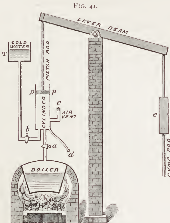
Newcomen Engine (Black).
