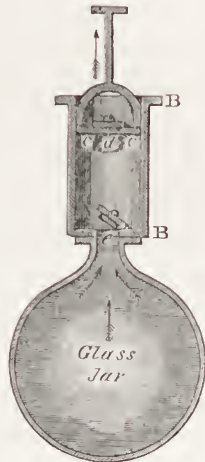
Air-pump (Knight).
