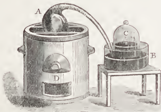
Lavoisier's Apparatus for Heating Mercury and making it take up Oxygen.
