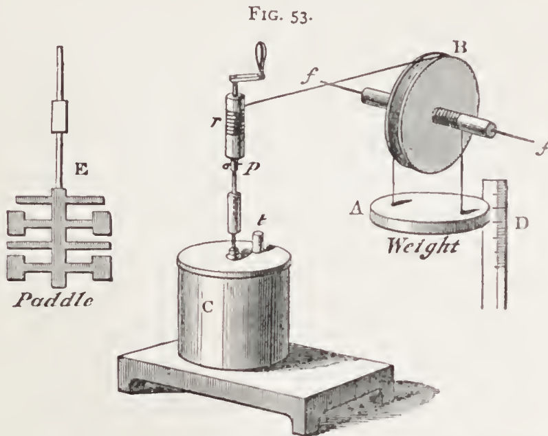
Joule's Experiment on the Conversion of Motion into Heat (Phil. Trans).
