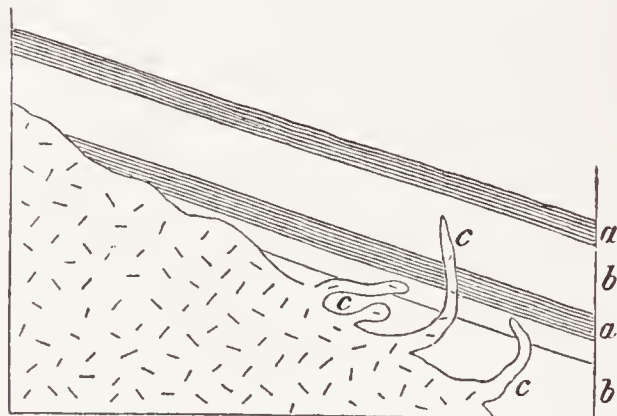
Granite Veins in Glen Tilt.
