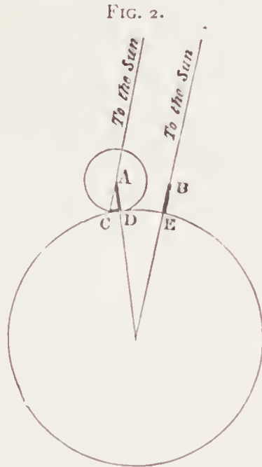
Diagram showing how Eratosthenes measured the circumference of the earth.
