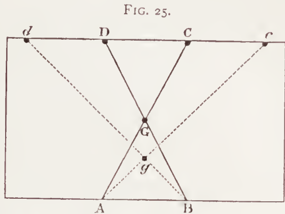
Diagram showing how the distance between the points D c and d c can be known without measuring them. G, A globe half-way between D c and A B. g, A globe three times as far from D c as from A B.
