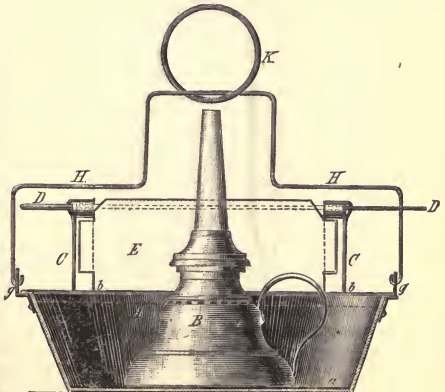
FIG. 68.—Trap-lantern of J. R. Stephens.
