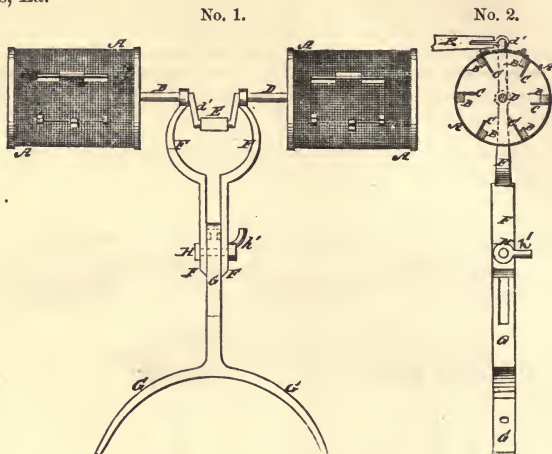
FIG. 59.—C. A. Levy's machine.
