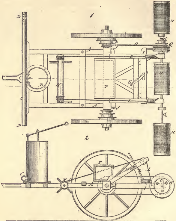
FIG. 61.—W. T. Robinson's combined sprinkler and duster.
