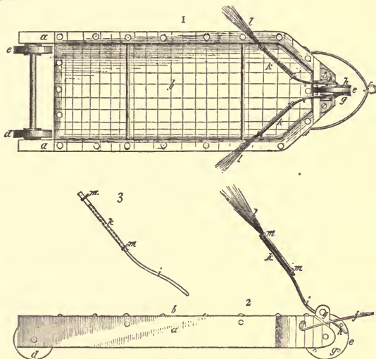
FIG. 63.—W. Ewing's machine.
