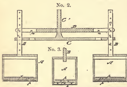
FIG. 57.—Willis' sifter.
