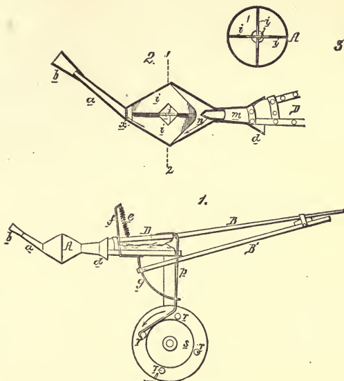
FIG. 53.—Allen's duster.
