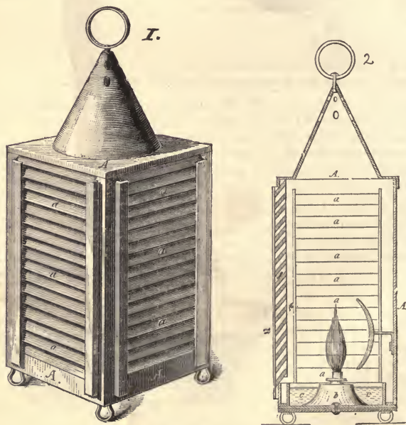
FIG. 69.—Trap-lantern of R. Pitman.
