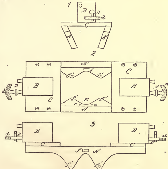
FIG. 53.—W. T. Willie's atomizer.
