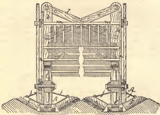
FIG. 62.—Helm's machine.
