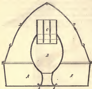
FIG. 71.—G. C. Cranston's lantern.
