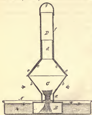
FIG. 73.—Byrne & Strunk's trap-lantern.
