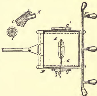
FIG. 54.—J. W. Johnson's machine.
