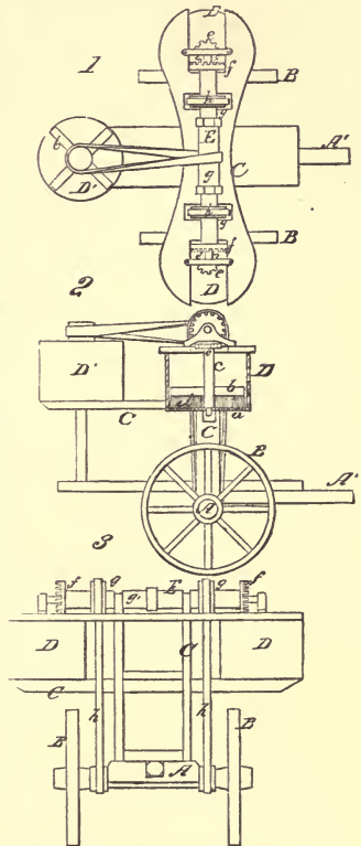
FIG. 60.—F. A. Eldridge's machine.
