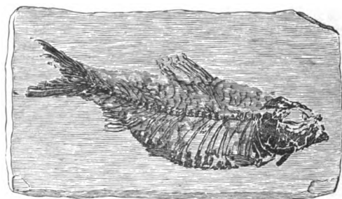
FIG. 46. — Clupea humilis . Eocene Shale. Wyoming. (Original.)
