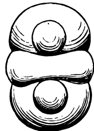
FIG. 9. Clay-Stones from the banks of the Connecticut River. (Original.)
