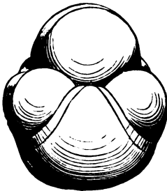
FIG. 9. Clay-Stones from the banks of the Connecticut River. (Original.)
