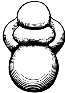
FIG. 10. Clay-Stones, foot of Mount Tom, Mass. (Original.)
