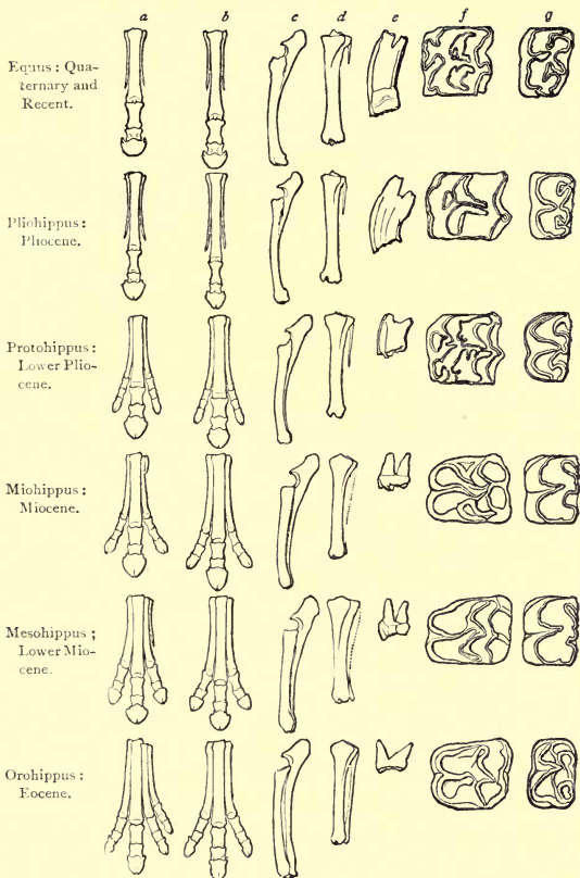
DIAGRAM ILLUSTRATING THE EVOLUTION OF THE HORSE.
