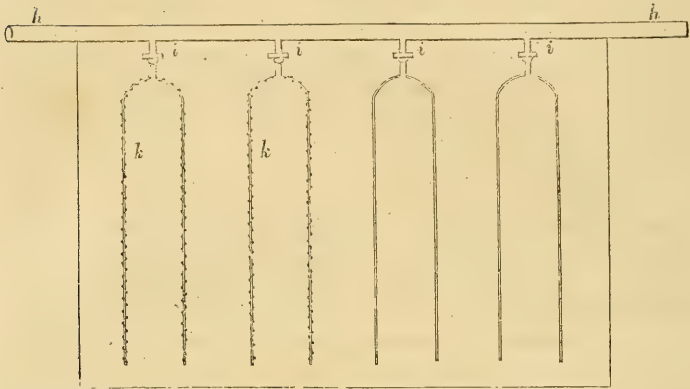
h, Pipe from water casks outside, continued on at back of centre bed. i, Small shoulders, soldered in, and stopcocks affixed. k, Copper tubes, which fit the shoulders, and are removable at pleasure. These are punctured laterally, to disperse the water.
