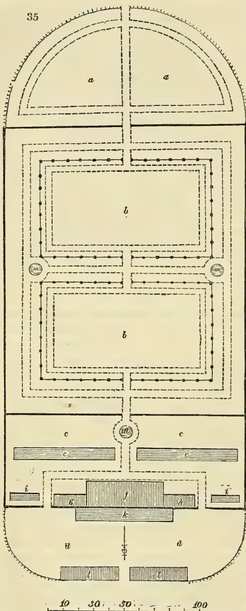
a a , Fruit-garden, and for potherbs. b b , Culinary department, with espaliers. c c , Forcing department. d d , Department for compost, mixing dung, &c. e e , Ranges for melons and cucumbers. f , Pine stove. g , Peach house. h , Vinery. i i , Pits. k , Back shed. l l , Mushroom sheds, or for other purposes. m m , Water basins, or places for pumps.
