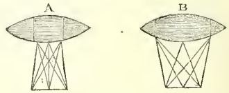
Diagram to illustrate angle of aperture.
