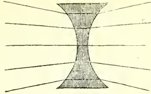
Rays slightly converging made to diverge.
