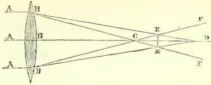
Diagram illustrative of chromatic aberration.
