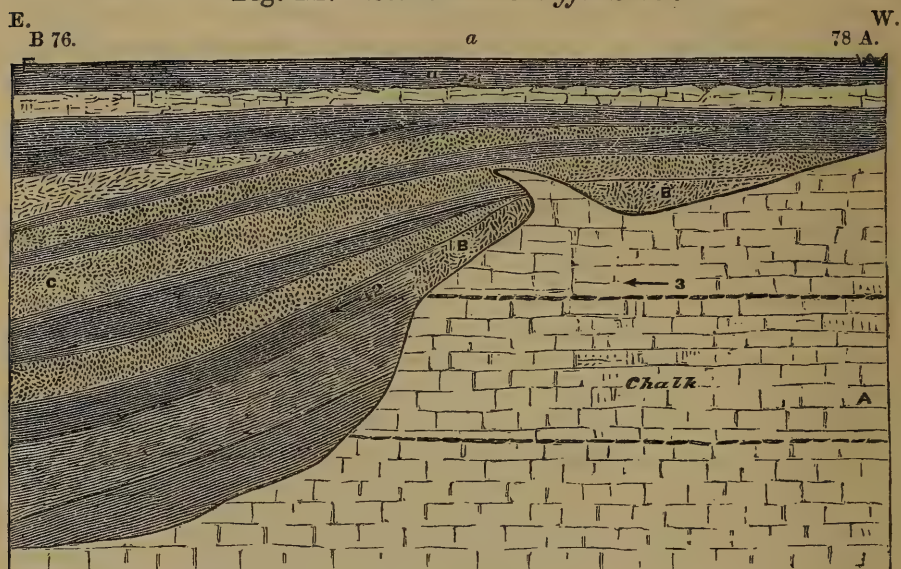
Fig. 22.—Section in Crayford Pit.
