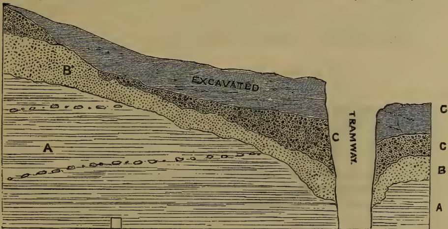
Fig. 24.—Section in Crayford Pit.
