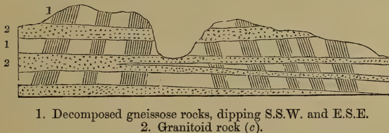
Fig. 2.—Granitiform rock in decomposed Gneiss, Suisgill.
