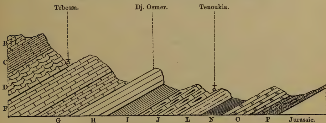
Fig. 4.—Section of the Cretaceous Beds of Algeria.
