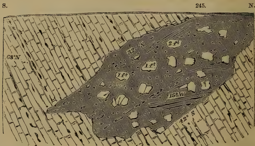
Fig. 33.— Section on Brading Down, Isle of Wight, showing blocks of Chalk in Gravel.
