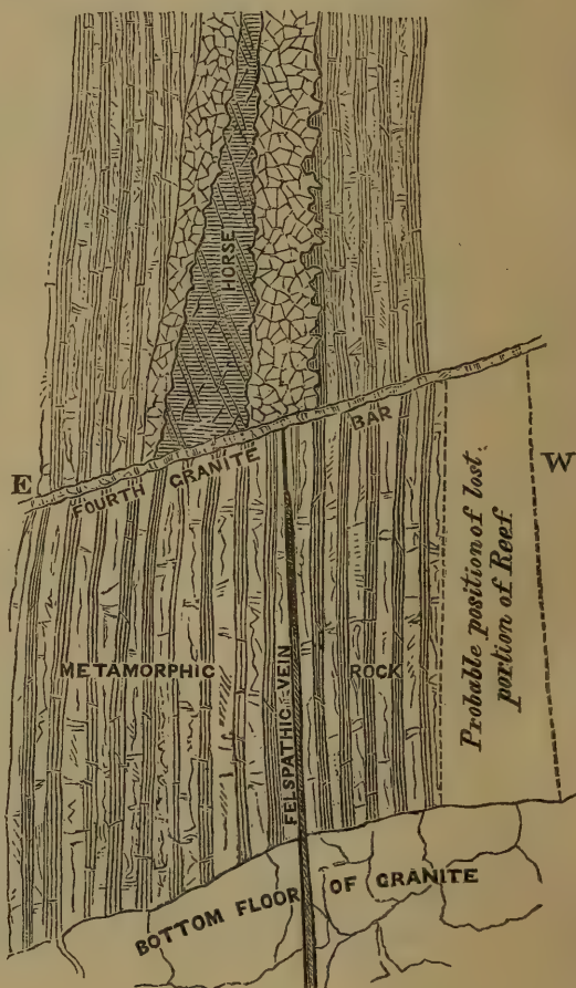
Fig. 7.—Cross Section, showing fourth Granite-vein cutting off the Reef (eastern and western veins with "Horse" between) and probable position of lost portion, also granite bottom floor and felspathic vein.
