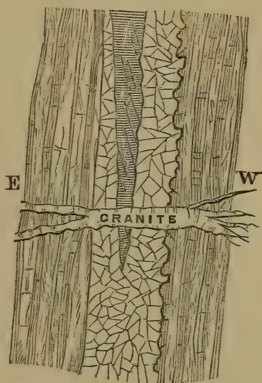
Fig. 5 b.—Cross section of the Reef along line a b of fig. 5 a.
