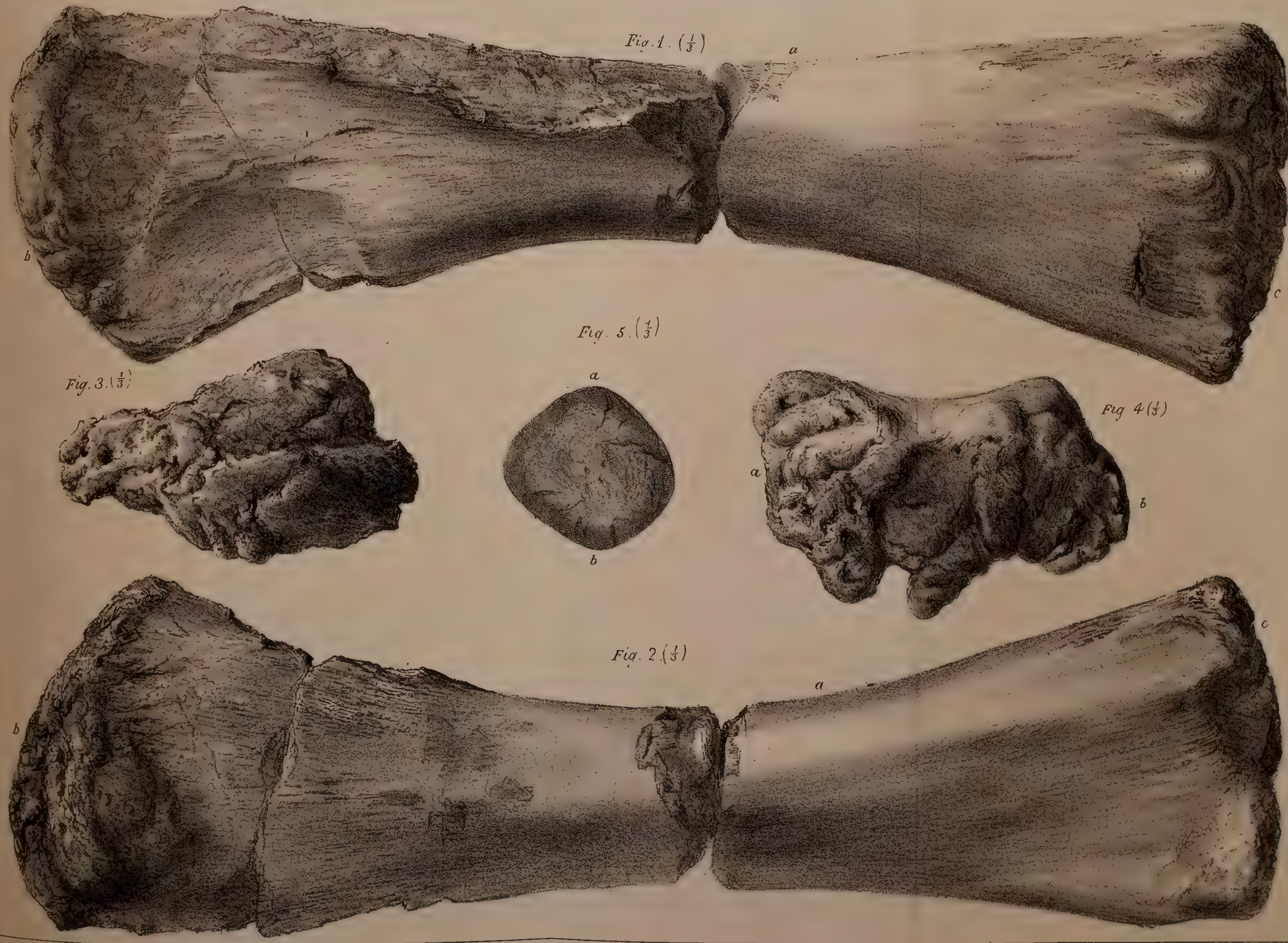
SAURIAN HUMERUS FROM KIMMERIDGE
