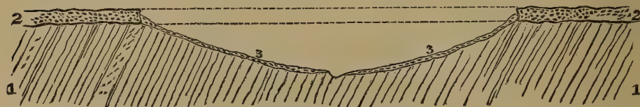
Fig. 4.— Valley-section, showing the Formation of "Tierra de flor" from "Moco de hierro."
