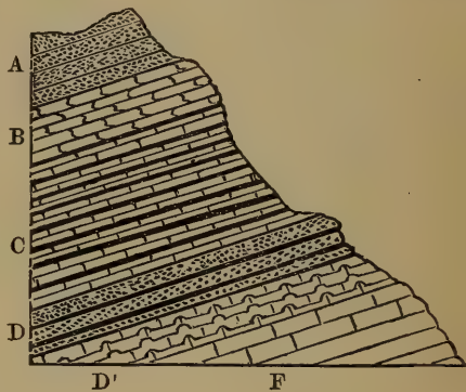
Fig. 3.—Section of the Freshwater Upper Cretaceous Beds of Fuveau.
