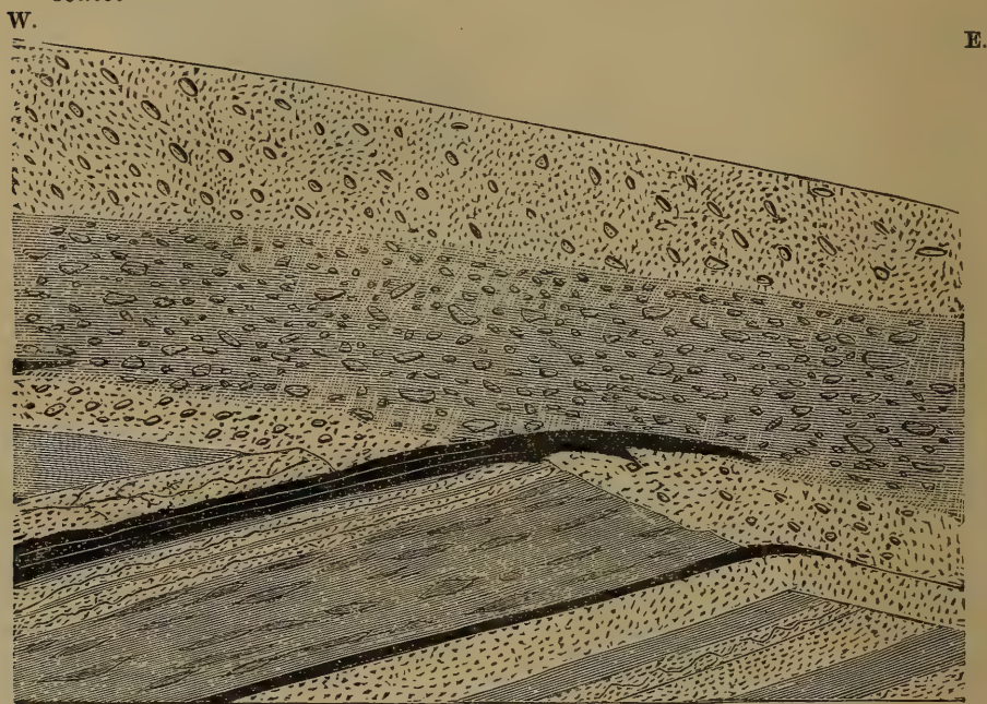
Fig. 8.—Section showing Coal-seams squeezed into drift during the deposition of the lowest gravel on Hirwain Common.—Natural scale.
