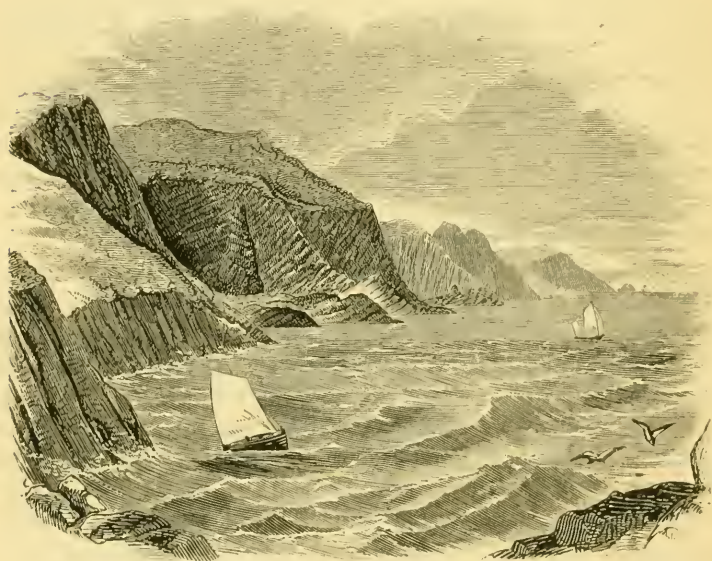
FIG. 4.— View of the cliffs of curved Silurian strata to the north-west of St Abb's Head.—See p. 13.
