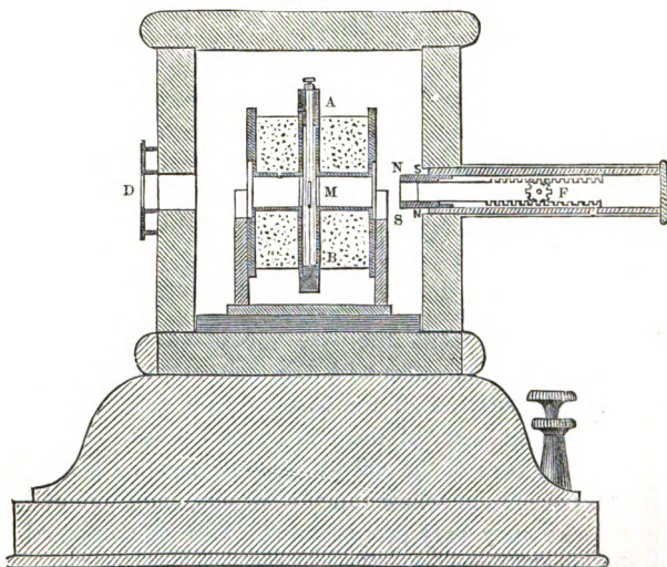
FIG. 98. Sectional Elevation.
