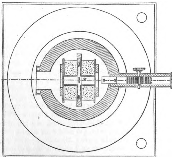
Sectional Plan.
