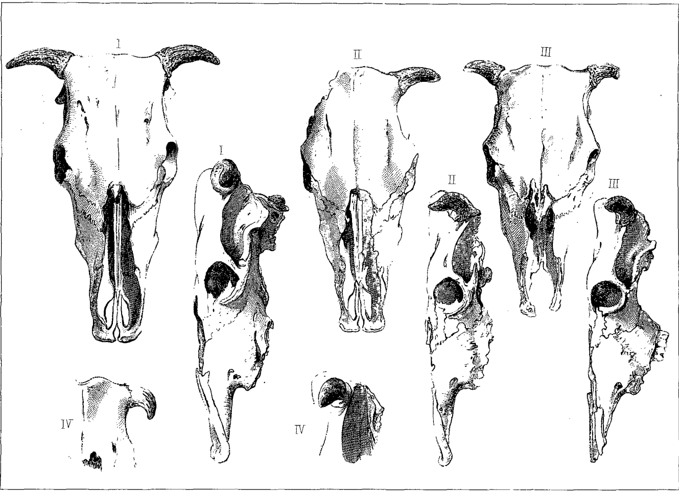
Skulls found with Roman Remains near Newstead, Roxburghshire, 1846-7.
