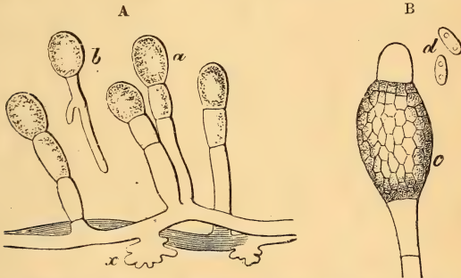
FIG. 376.—The vine-mildew : A, the Fungus Oidium Tuckeri ; a the oïdium-spores (conidia) becoming detached ; x the organs of attachment ; b a germinating spore (× 400). B, c the so-called cicinobulus-fruit [or cyst], a later form of fructification of the vine-mildew ; d its spores. (× 450.)
