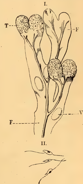
FIG. 389.— Fucus vesiculosus ; I. \tau thallus; T fructification; V air-bladder (natural size); II. antherozoids (greatly magnified).
