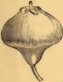
FIG. 241.—Urceolate corolla of Vaccinium Myrtillus (magnified).
