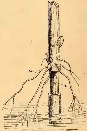
FIG. 348.—A cutting from which a ring of bark has been removed placed in water; from above this place a adventitious roots w are developed.
