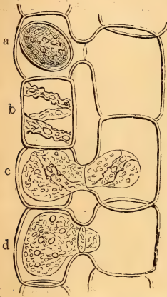
FIG. 54.—Conjugation and spore-formation of Spirogyra quinina : a a mature spore; b a cell not yet conjugated; c, d successive stages of conjugation. ( \times 320 .)
