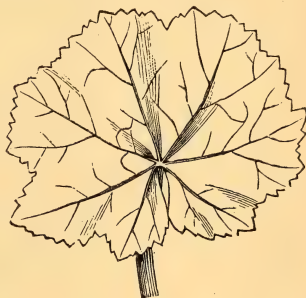
FIG. 155.—Orbicular leaf of Malva rotundifolia .
