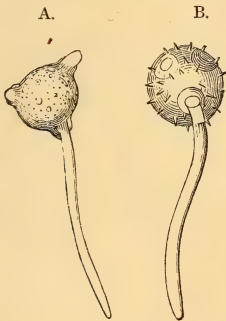
FIG. 358.—Pollen-grains putting out their pollen-tube: A Dipsacus Fullonum ; B Cucurbita .
