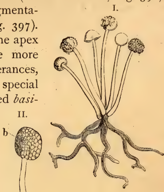
FIG. 396.— Ascophora Mucedo : I. an entire plant with six sporangia in different stages of development (strongly magnified); II. single sporangium with spores b ( \times 200 ).
