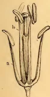
FIG. 529. — Tetradynamous stamens and pistil of Brassica nigra ; a shorter, b longer stamens.
