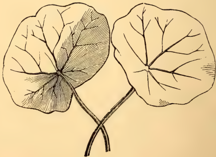
FIG. 162.—Peltate leaf of Tropaeolum .
