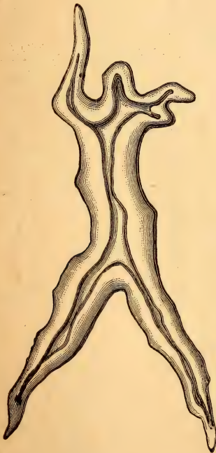
FIG. 17.—Branched bast-cell of the larch. ( \times 200 .)
