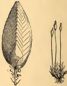
FIG. 431.— Sphagnum acutifolium ; I. part of the stem with two sporogonia a and four antheridial receptacles b (after Schimper, \times 3 ); II. an antheridial receptacle separated, with the perigonal leaves removed from the lower part so as to expose the stalked globular antheridia (more strongly magnified).
