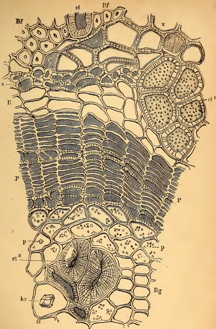
FIG. 67.—Transverse section through the innermost layer of the bark of the oak; P P layer of periderm consisting of thick-walled cells filled with a homogeneous red mass; pp parenchymatous cells with starch-grains; st 1 parenchymatous cells with moderately thickened, st 11 with strongly thickened walls; Bg bast-vessels or sieve-tubes; Bf bast-tubes; B parenchyma and bast-vessels; kr a large parenchymatous cell containing a crystal; x a periderm-like tissue. (x 440.)
