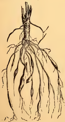
FIG. 106.—Tuberous fasciculated root of Spiraea filipendula .
