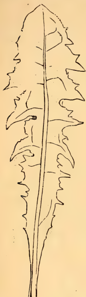
FIG. 175.—Runcinate leaf of the dandelion.
