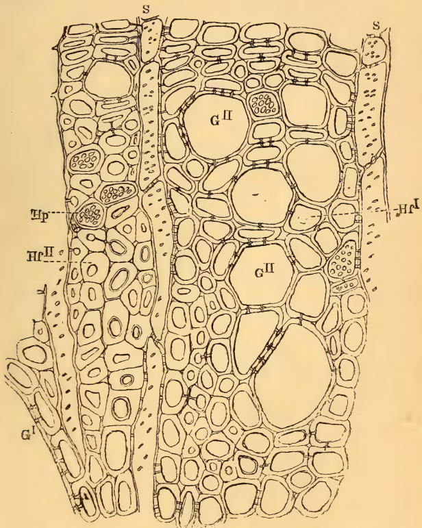
FIG. 475. — Transverse section through the wood of the oak; Hf' thin-walled, Hf'' strongly thickened wood-fibres; Hp' parenchyma of the xylem; s fibres of the 'silver-grain'; G' small vessels; adjoining G' is a very large vessel, the size of which is only slightly indicated by the curved border-line.
