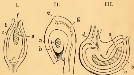
FIG. 300.—I. Orthotropous; II. anatropous; III. campylotropous ovule; a nucleus with the embryo-sac coloured dark; b primine; c secundine; de chalaza; f micropyle (represented diagrammatically).
