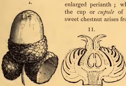
FIG. 303.—I. Acorn of Quercus sessiliflora with two empty cupules; II. longitudinal section through the fertilised pistillate flower, with the cupule in an early state.
