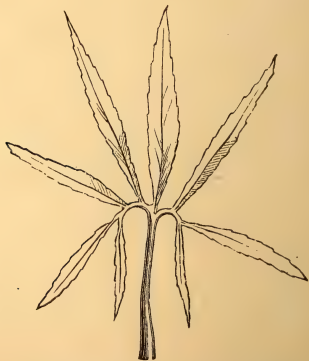
FIG. 183.—Pedate leaf of the Christmas rose, Helleborus niger .
