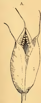
FIG. 290.—Basilar style of Alchemilla (magnified).
