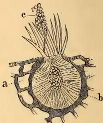
FIG. 406.— Puccinia graminis : a b cells of the leaf of the host ( Berberis vulgaris ); the spermatia c are escaping from the sporogonium (after De Bary, \times 200 ).
