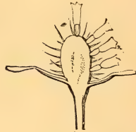
FIG. 218.—Receptacle of Anthemis arvensis with paleæ between the flowers.
