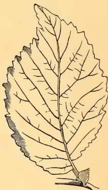
FIG. 145.—Leaf of the elm, with small stipules.
