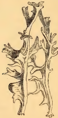
FIG. 415.— Cetraria islandica , a Fruticose Lichen; the margin of the thallus is fringed, and bears spermogonia on the edge of the fringe; there are no apothecia.
