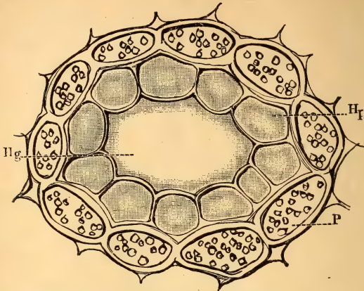
FIG. 79.—Transverse section through a mature resin-passage of Abies excelsa ; the cavity Hg as well as the thin-walled cells Hg are filled with a semi-fluid resin, while the thick-walled compressed cortical cells P still contain small quantities of starch. ( \times 800 .)
