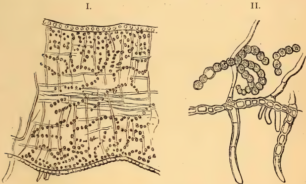
FIG. 412.—I. Longitudinal section through the thallus of a Gelatinous Lichen, Maiotium Hildenbrandii ( \times 190 ); II. piece of a very thin section through the under side with moniliform chains of gonidia (after De Bary, \times 390 ).
