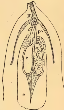
FIG. 367.—Fertilisation of Abies excelsa : p pollen-grains; ps pollen-tubes; c two corpuscles in the embryo-sac e. (x 60.)
