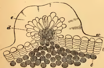
FIG. 80.—Transverse section of a resin-gland from a young birch-twig; a epidermal cells; b a subjacent layer of cork; c collenchymatous cortical tissue; d the papillæ of the gland which have secreted the solid resin e . ( \times 100 .)
