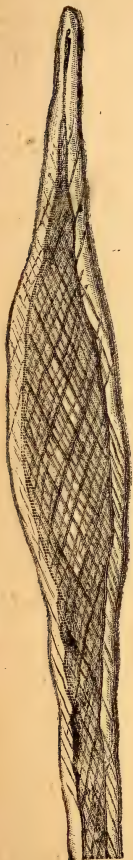
FIG. 26.—Bast-cell of Cynanchum vincetoxicum , with intercrossing spiral striations. ( \times 370 .)
