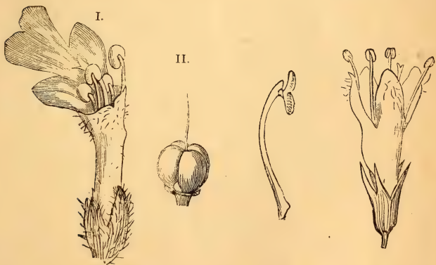
FIG. 490.— Ajua reptans ; I. flower; II. pistil (magnified).
