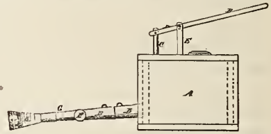
Fig. 56.—THE GOODIN SPRINKLER: side view.
