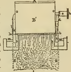
FIG. 42.—HURD BLOWER: rear view.
