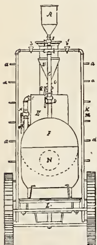
FIG. 77.—THE STEINMANN VAPORIZER: rear view.
