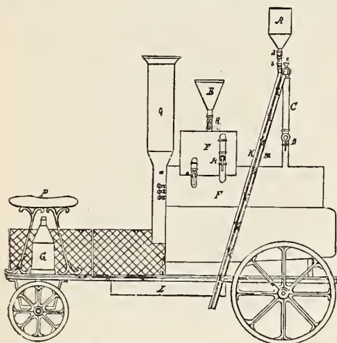
FIG. 76.—THE STEINMANN VAPORIZER: side elevation.
