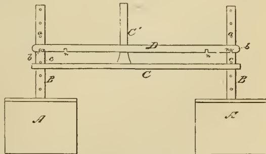
FIG. 38.—THE WILLIE DUSTER: front view.
