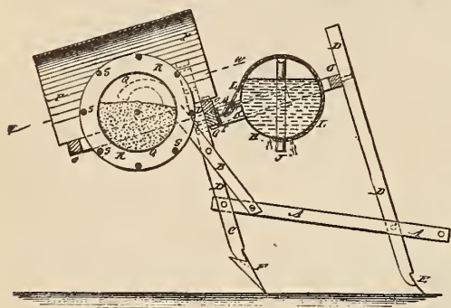
FIG. 49.—THE TAYLOR DUSTING AND SPRINKLING MACHINE.
