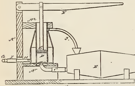
FIG. 57.—THE YEAGER SPRINKLER: side view.
