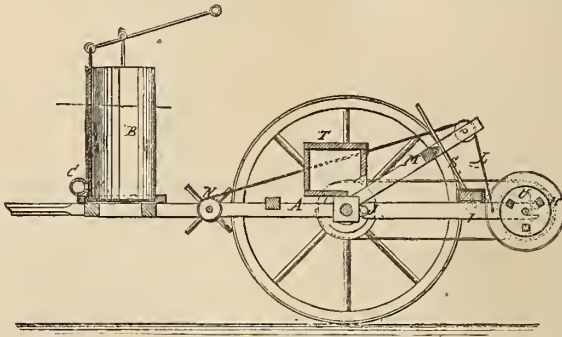
FIG. 44.—THE ROBINSON DUSTER AND SPRINKLER: longitudinal section.
