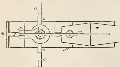
FIG. 58.—THE YEAGER SPRINKLER: top view.
