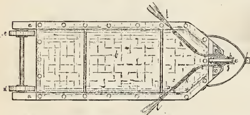
FIG. 29.—EWING BRUSHING-MACHINE: Top view.
